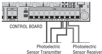
IR2 Functionality
