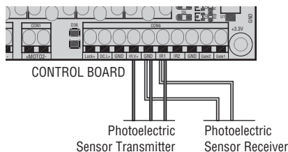
IR1 Functionality
